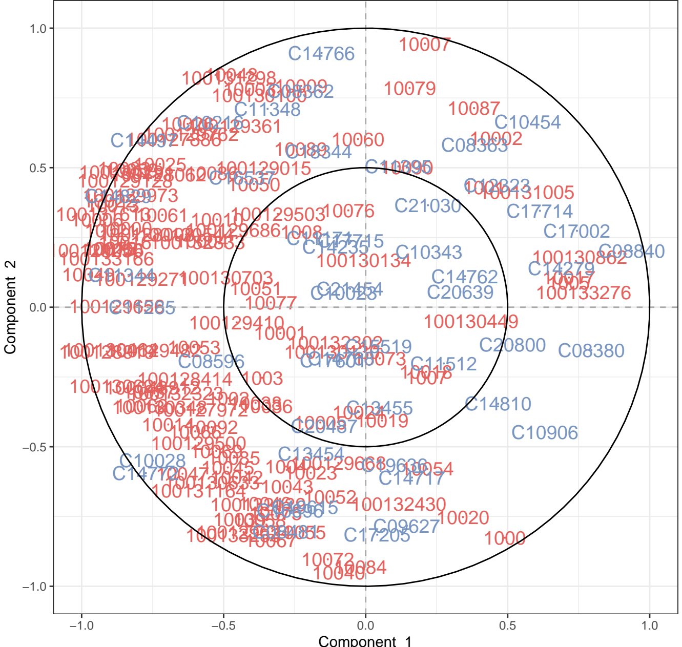
Correlation Circle Plot
