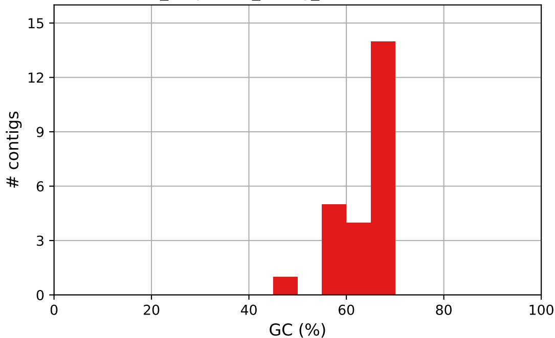
virus_suspected_contig_filtered GC content
