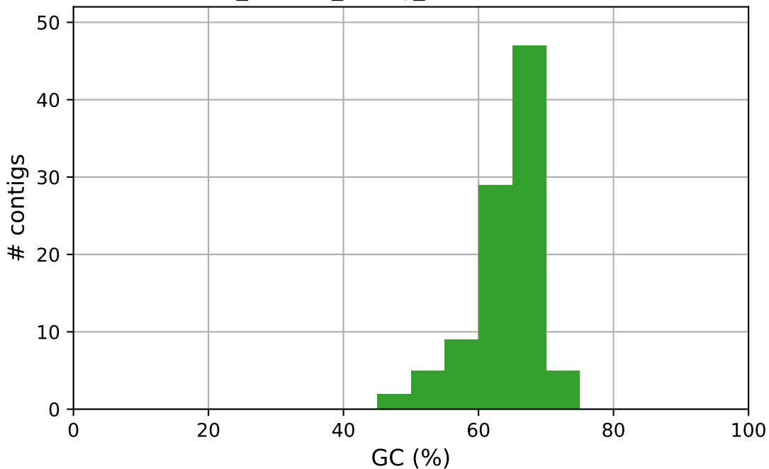
virus_denovo_contig_filtered GC content
