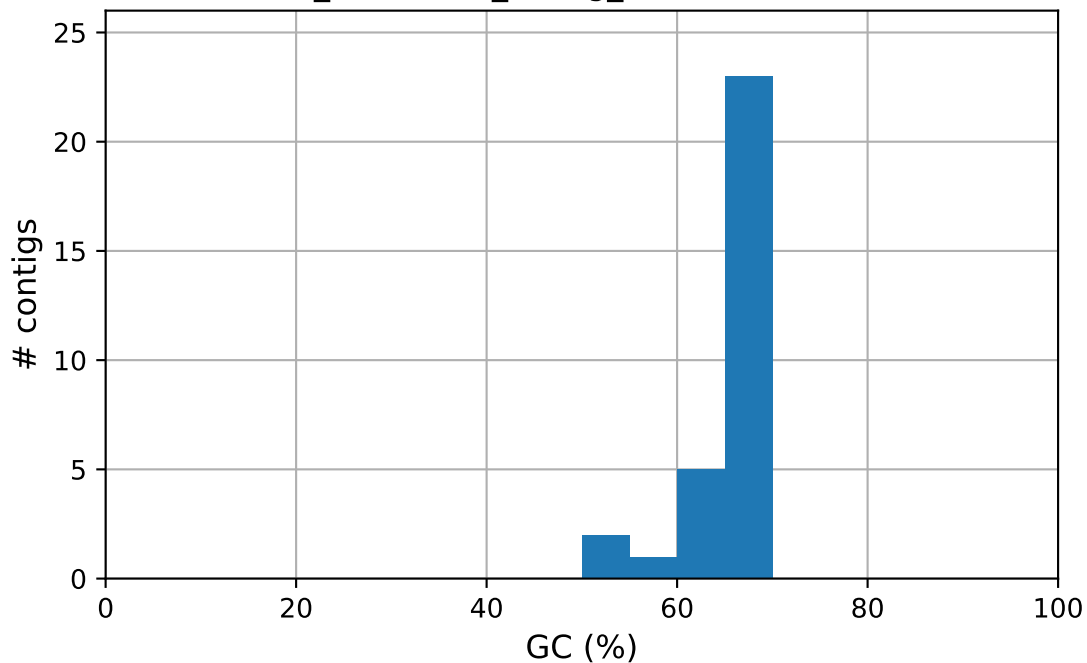
virus_confirmed_contig_filtered GC content
