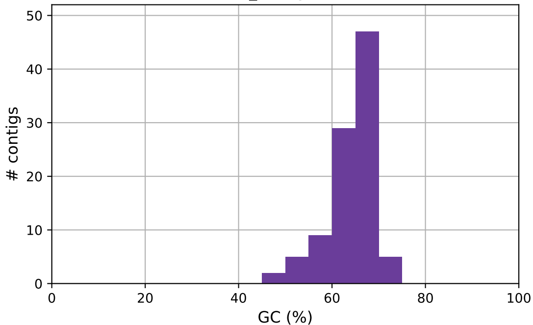
combined_contig GC content
