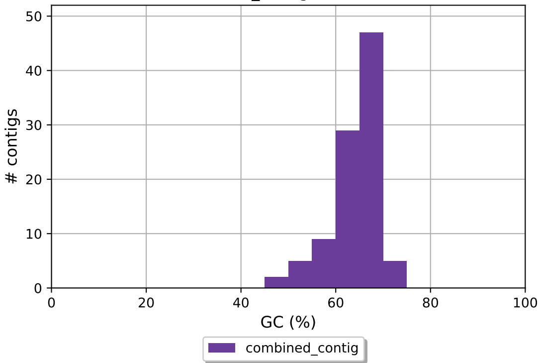
combined_contig GC content
