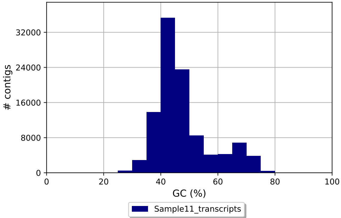
Sample11_transcripts GC content
