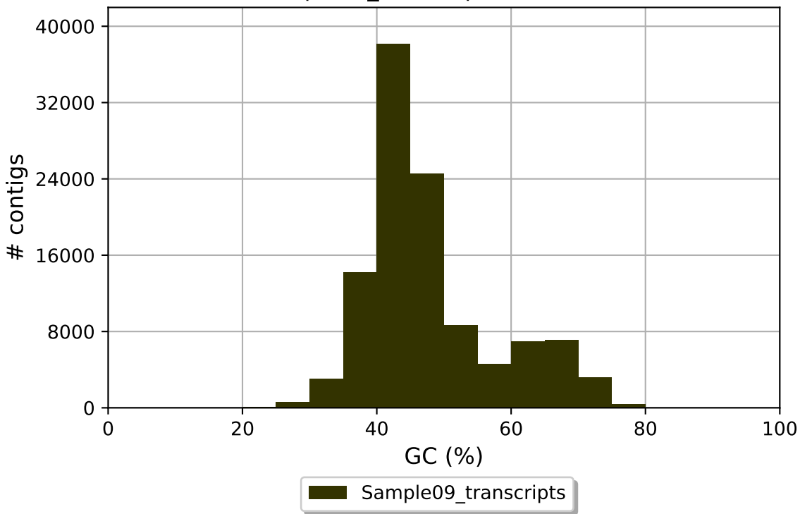
Sample09_transcripts GC content
