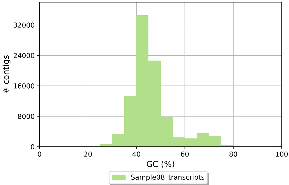
Sample08_transcripts GC content
