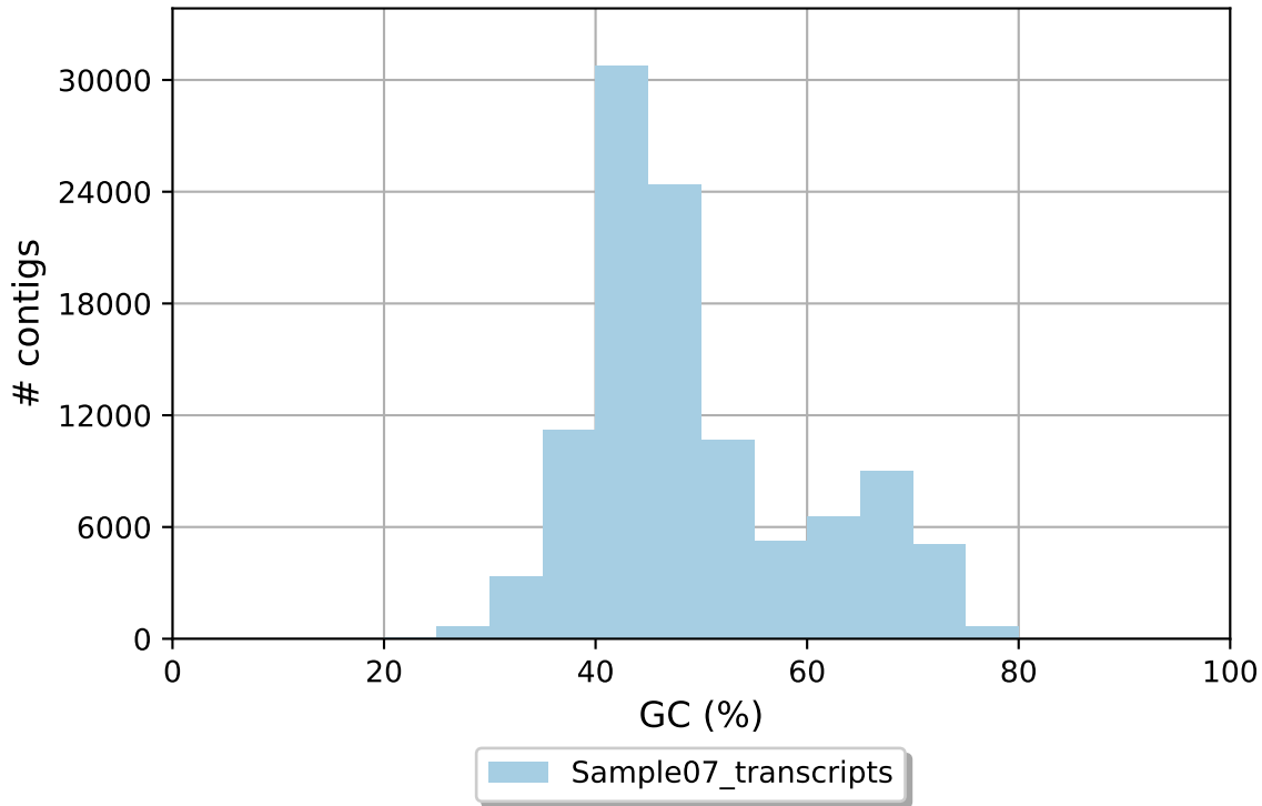
Sample07_transcripts GC content
