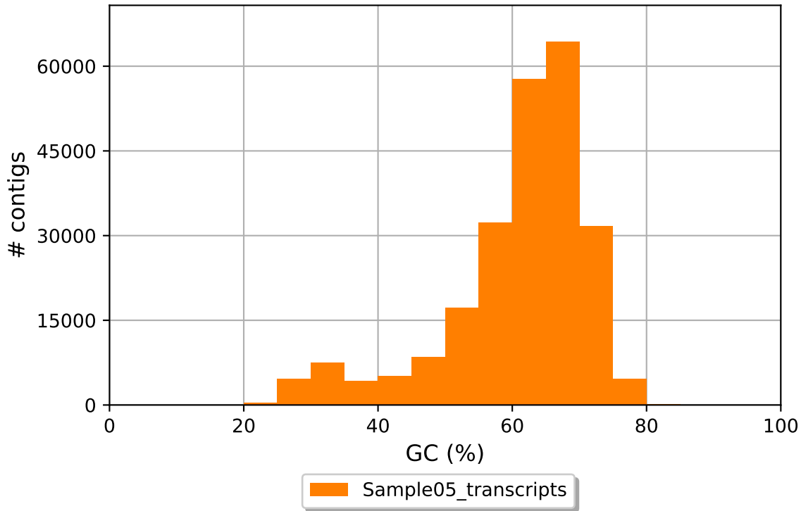
Sample05_transcripts GC content
