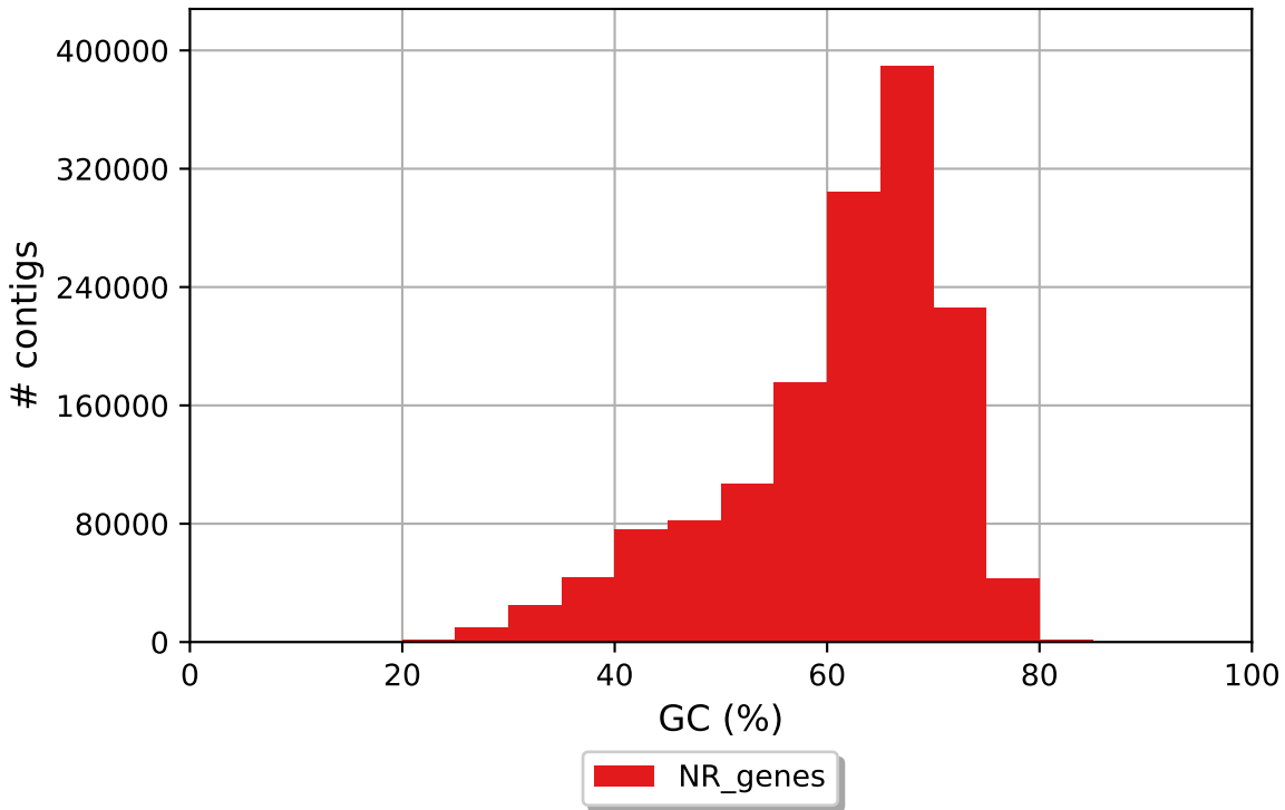
NR_genes GC content
