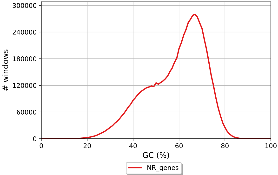
GC content
