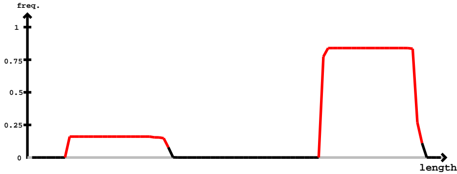
hsa-let-7d-3p
